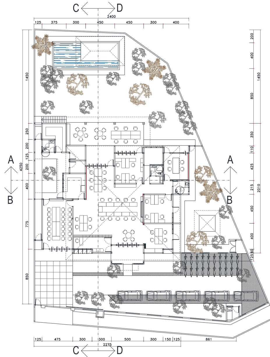
DENAH DESIGN LANTAI 1
