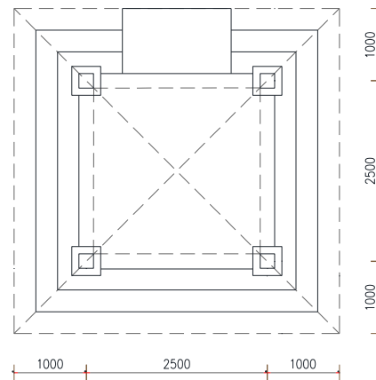
DENAH
