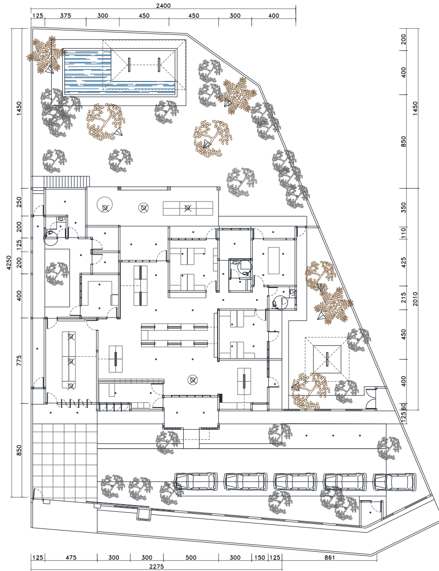
DENAH LAMPU LANTAI 1
